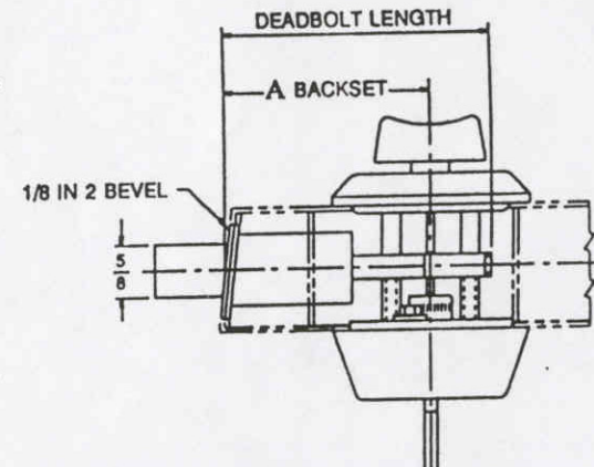
DRIVE-IN DEADBOLT SHOWN
