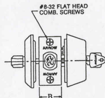
STRAIGHT FRONT SHOWN
